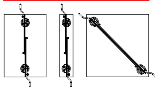
SLAB TABLE Ref. 18935 SLAB TABLE VERSA-TILE Ref. 18984
